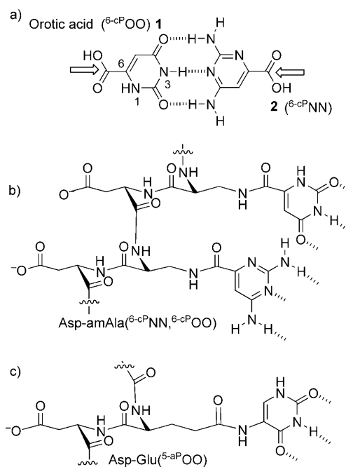
Figure 1. a) The tridentate Watson–Crick-type base pair between orotic acid ( 6-cP OO, 1 ) and its 2,4-diamino counterpart ( 6-cP NN, 2 ); b) Idealized conformation of Asp-amAla oligo-dipeptide backbone tagged with 6-cP OO and 6-cP NN—derived from the type of conformational reasoning [7] applied in the case of c). c) Asp-Glu oligo-dipeptide tagged with 2,4-dioxo-5-aminopyrimidine ( 5-aP OO). [2b]
