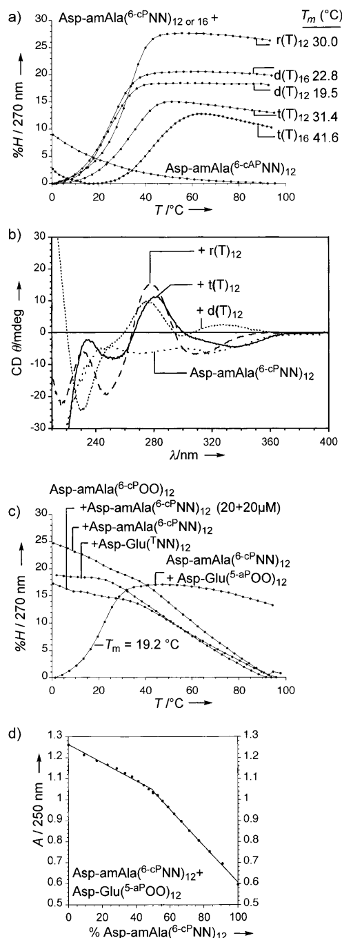
Figure 3. Base-pairing behavior of Asp-amAla( {}^6\text{-cPNN} ) oligo-dipeptides. a) UV spectroscopic T_m curves demonstrating strong pairing with (r) RNA, (d) DNA, and (t) TNA sequences containing thymine. b) CD spectral comparison of Asp-amAla( {}^6\text{-cPNN} ) 12 and the corresponding duplexes formed with r(T) 12 , d(T) 12 , and t(T) 12 . c) UV spectroscopic T_m curves documenting pairing behavior in the inter- and intra- oligo-dipeptide systems. d) Job plot showing the 1:1 ratio of the pairing partners in the intra-system homo-duplex formed at 0 °C (see Table S2, entry 31 in the Supporting Information). Measurement conditions: see caption for Figure 3.
