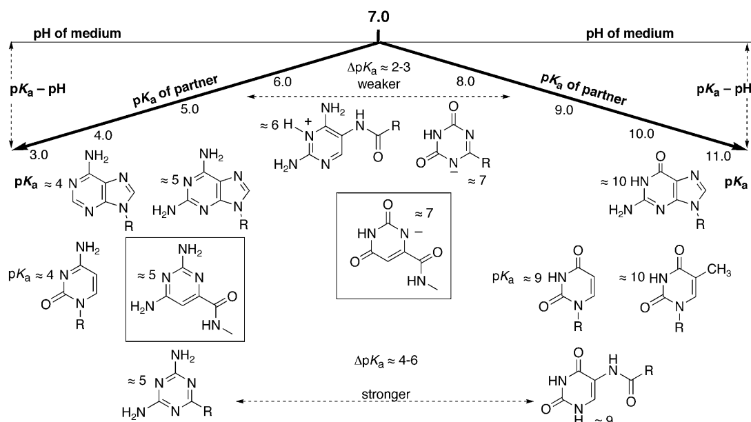
Figure 4. Correlation of the pK_a value of the base-pairing partners with their base-pairing strength (aq. neutral conditions). The pK_a values below 7 are for the conjugate acid of the heterocycles. The canonical nucleobases and strongly base-pairing (potentially natural) heterocycles have pK_a values at least 2–3 units away from the pH of the medium, whereas the weakly pairing heterocycles have pK_a values which are closer.
