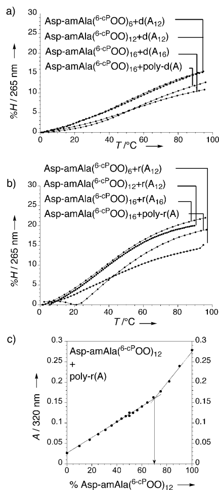
Figure 2. Weak base pair interactions of Asp-amAla( 6\text{-cP}\text{OO} ) oligomers. UV spectroscopic T_m curves of Asp-amAla( 6\text{-cP}\text{OO} ) oligomers documenting a) no pairing with DNA oligomers and b) very weak pairing with RNA oligomers. c) Job plot showing the 2:1 ratio of the pairing partners in the homo-duplex formed at 0°C. Measurements were made with total concentration of approximately 10 \mu\text{M} (1:1) in 1 M NaCl, 10 mM aq. \text{NaH}_2\text{PO}_4 , 0.1 mM \text{Na}_2\text{EDTA} , pH 7.0. No self pairing was observed for individual partner strands.
